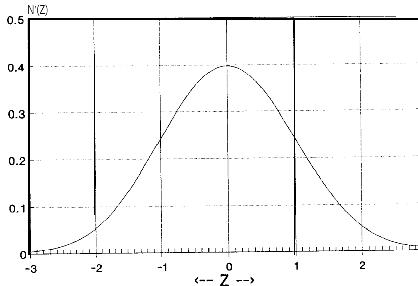
Figure 3-7 The Normal Probability density function.
