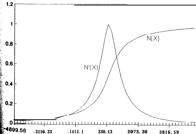
figure 4-10 Adjustable distribution fit to the 232 trades.
