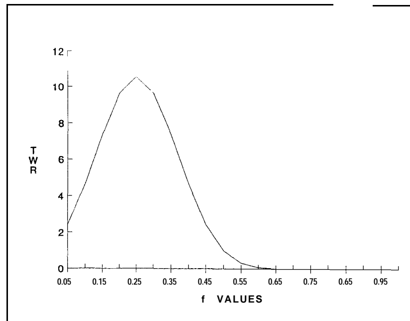
Figure 1-1 20 sequences of +2, -1.
