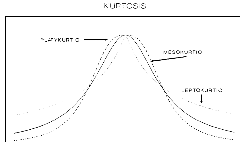
Figure 3-4 Kurtosis.
