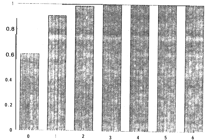
Figure EI 1 Cumulative probability functions for the Poisson Distribution (L = .5).
