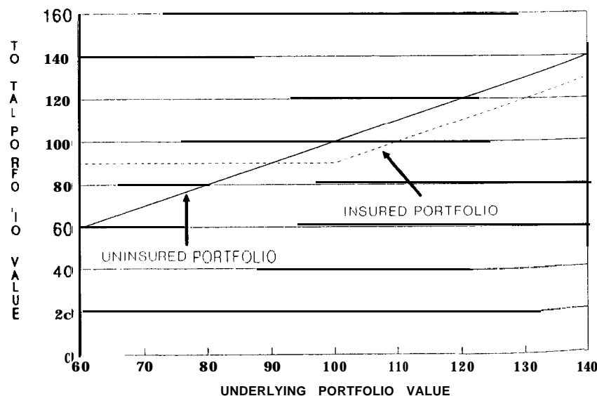
Figure 8-2 Portfolio insurance.
