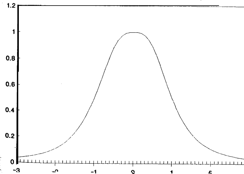
Figure 4-4 LOC = 0 SCALE = 1 SKEW = 0 KURT = 3.
