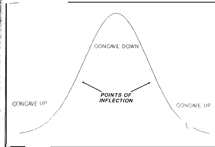
Figure 4-1 Points of inflection on a bell-shaped distribution.
