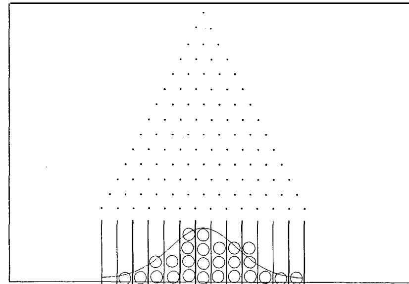
Figure 3-5 Galton's board.
