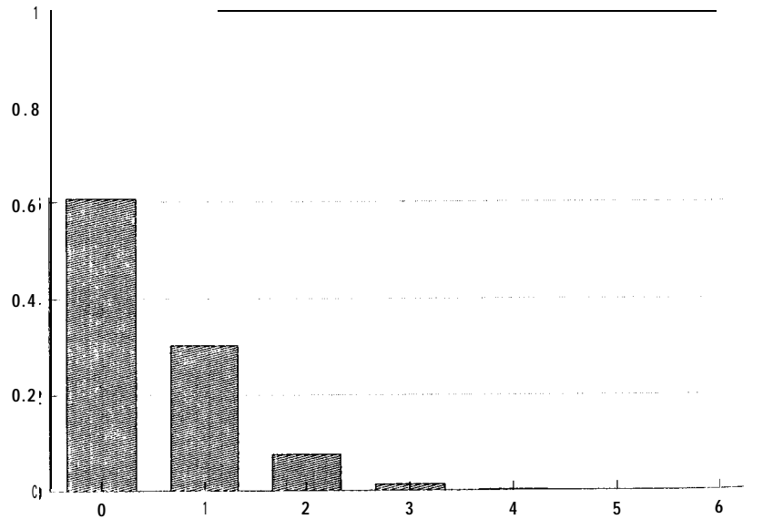
Figure B-I 0 Probability density functions for the Poisson Distribution (L = .5).
